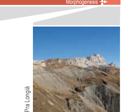
Pra Longià Erosion shapes the Dolomites
