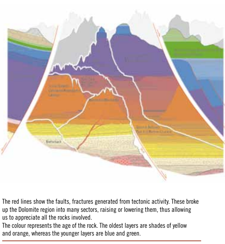
Pra Longià Erosion shapes the Dolomites
