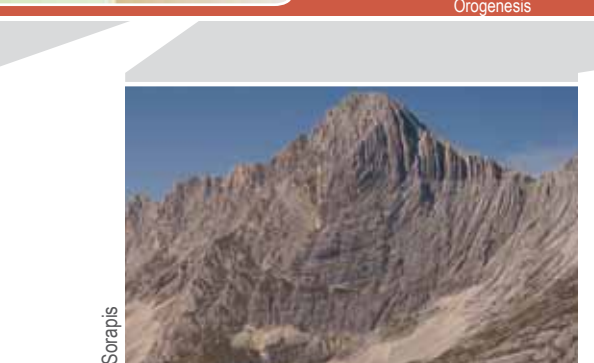
Sorapis Europe and Africa collide: the rocks deform
