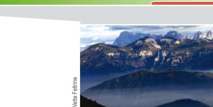
Vette Feltrine Everything sinks: an ocean is created
