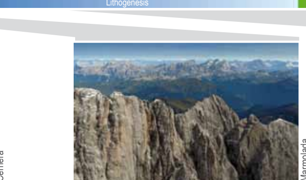
Marmolada Volcanoes are set, islands merge
