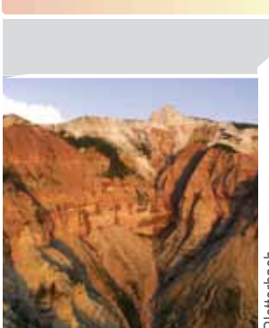
Bletterbach Broad plains and shallow seas
